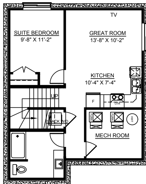
Alt. Legal Secondary Suite 635 Sq Ft
