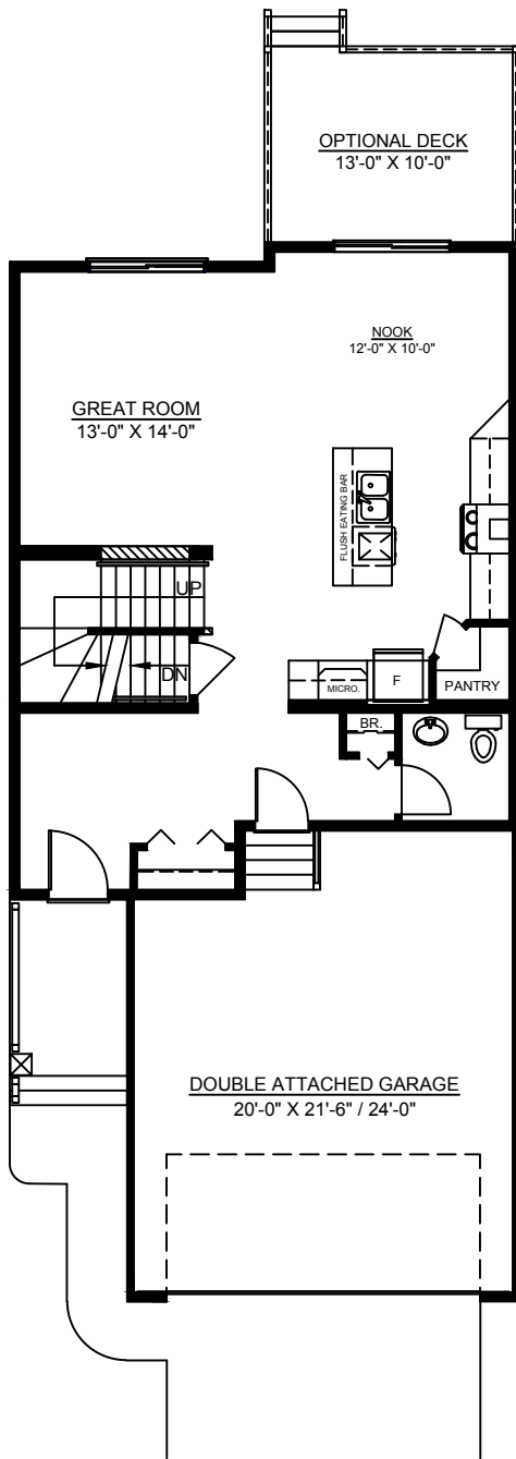
Main Floor 809 Sq Ft
