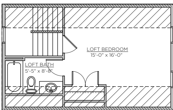
Optional Loft Development "B" 418 Sq Ft
