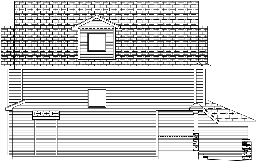
RIGHT ELEVATION "F"
