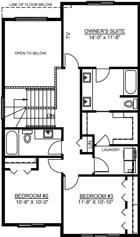
Alternate Upper Floor (Open to Below) 946 Sq Ft
