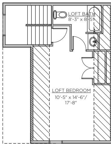
Optional Loft Development "F" 454 Sq Ft
