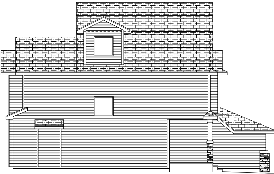
RIGHT ELEVATION "D"
