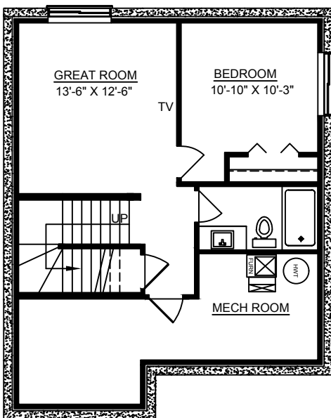
Alt. Lower Development 452 Sq Ft
