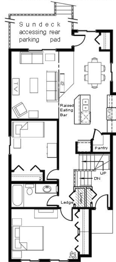
MAIN FLOOR MODEL "A" 1000 SQ. FT.
