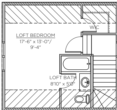
Optional Loft Development "B" 372 Sq Ft
