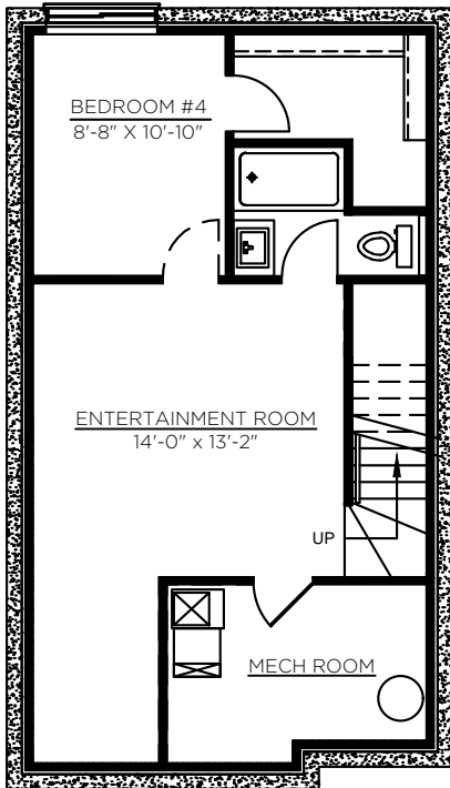
Optional Lower Level Development 520 Sq Ft
