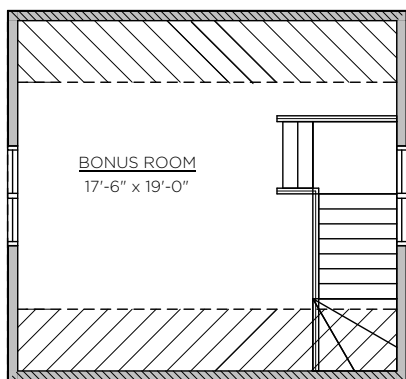
Optional Loft Development "A" 372 Sq Ft
