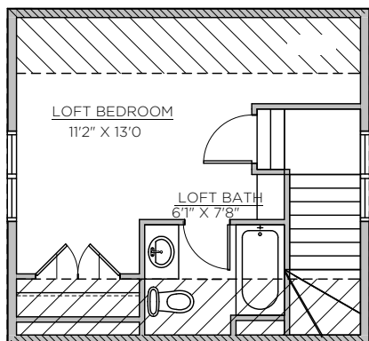
Optional Loft Development "C" 372 Sq Ft
